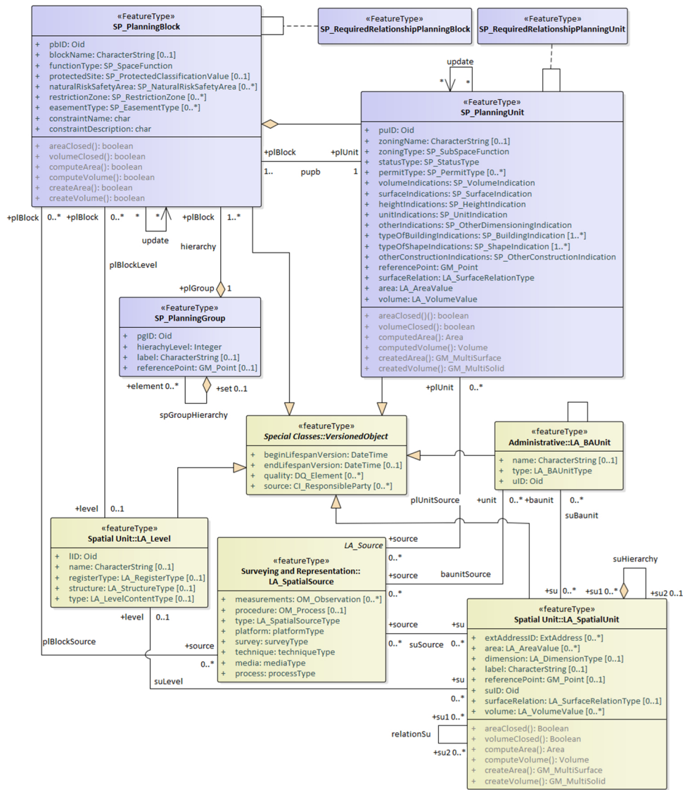
Fig. 12. Classes in spatial planning package and their relationship with LA_SpatialUnit class and VersionedObject class to construct 4D (3D + time) urban planning.
